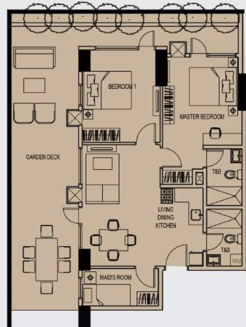
2G-1 FLOOR PLAN 120.48 SQ.M
